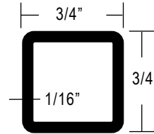
E-8771BK,EA,MF .093 Radii
