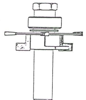
Light weight cap cutter head
