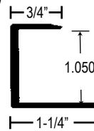
E-494 EA, MF 12' CAP For Capping edge of Decking
